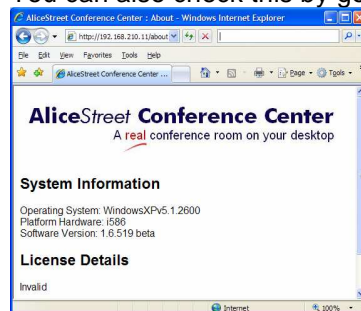
Figure 1 – About window
